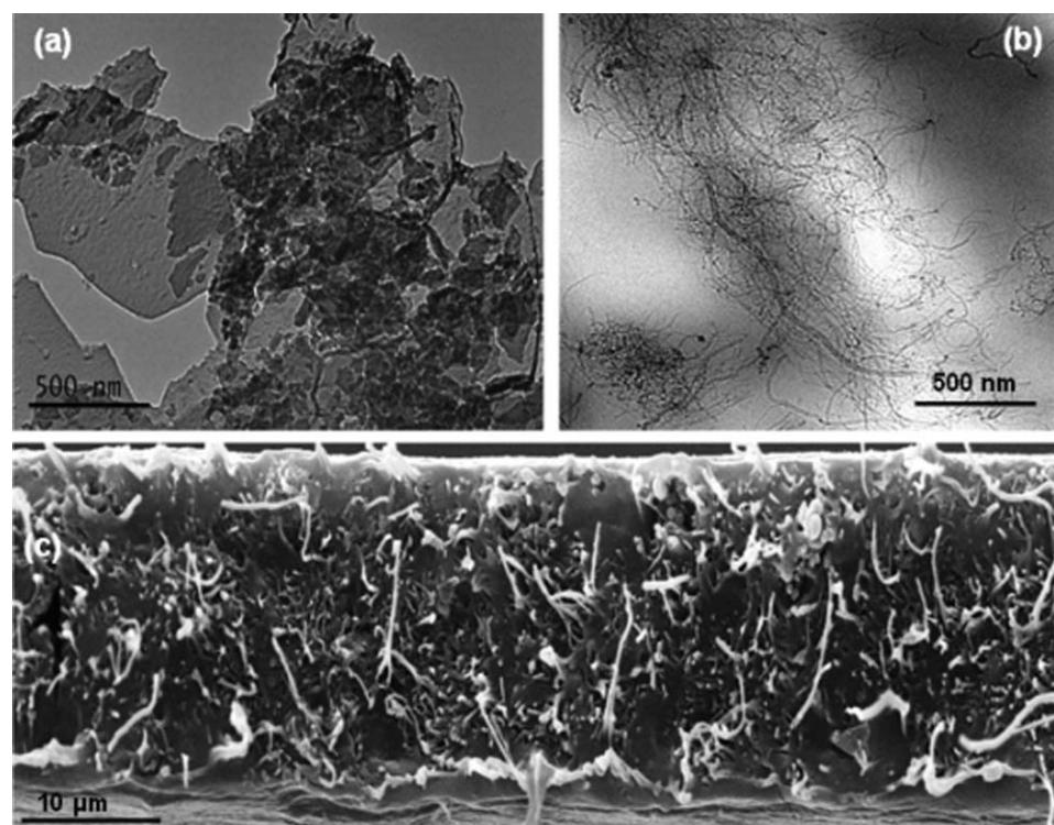
Figure 1. TEM and SEM analysis of the cross sections of composite films: (a,b) TEM micrographs of PLA/GNP/MWCNT and PP/MWCNT films, respectively, in magnification \times 10,000 ; and (c) SEM micrograph of the PLA/GNP/MWCNT film, in magnification \times 1000 .
