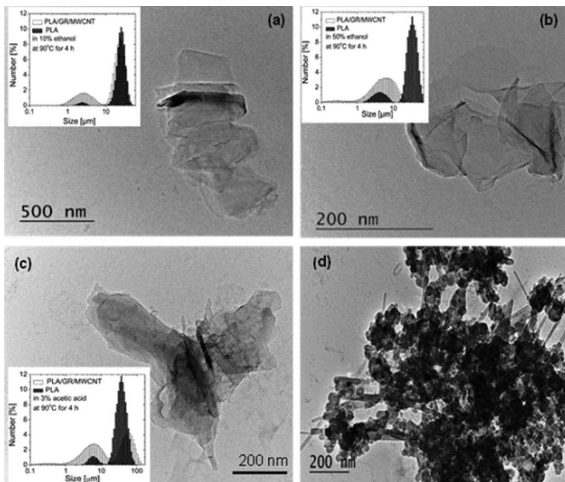
Figure 2. TEM micrographs of dried migrants from PLA/GNP/MWCNT film after high-temperature migration test (at 90 °C for 4 h): (a) in 10% ethanol; (b) in 50% ethanol; (c,d) in 3% acetic acid. Insets: size distribution histograms of migrants from the neat PLA (dark bars) and PLA/GNP/MWCNT films (light bars) in the liquid food simulants.
